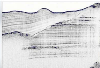
Subbottom Profiler record
