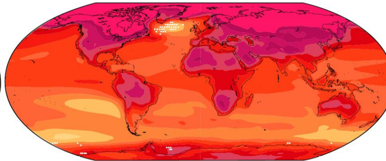
RCP8.5 2081-2100
