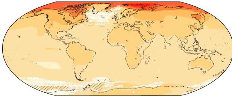
RCP2.6 2081-2100
